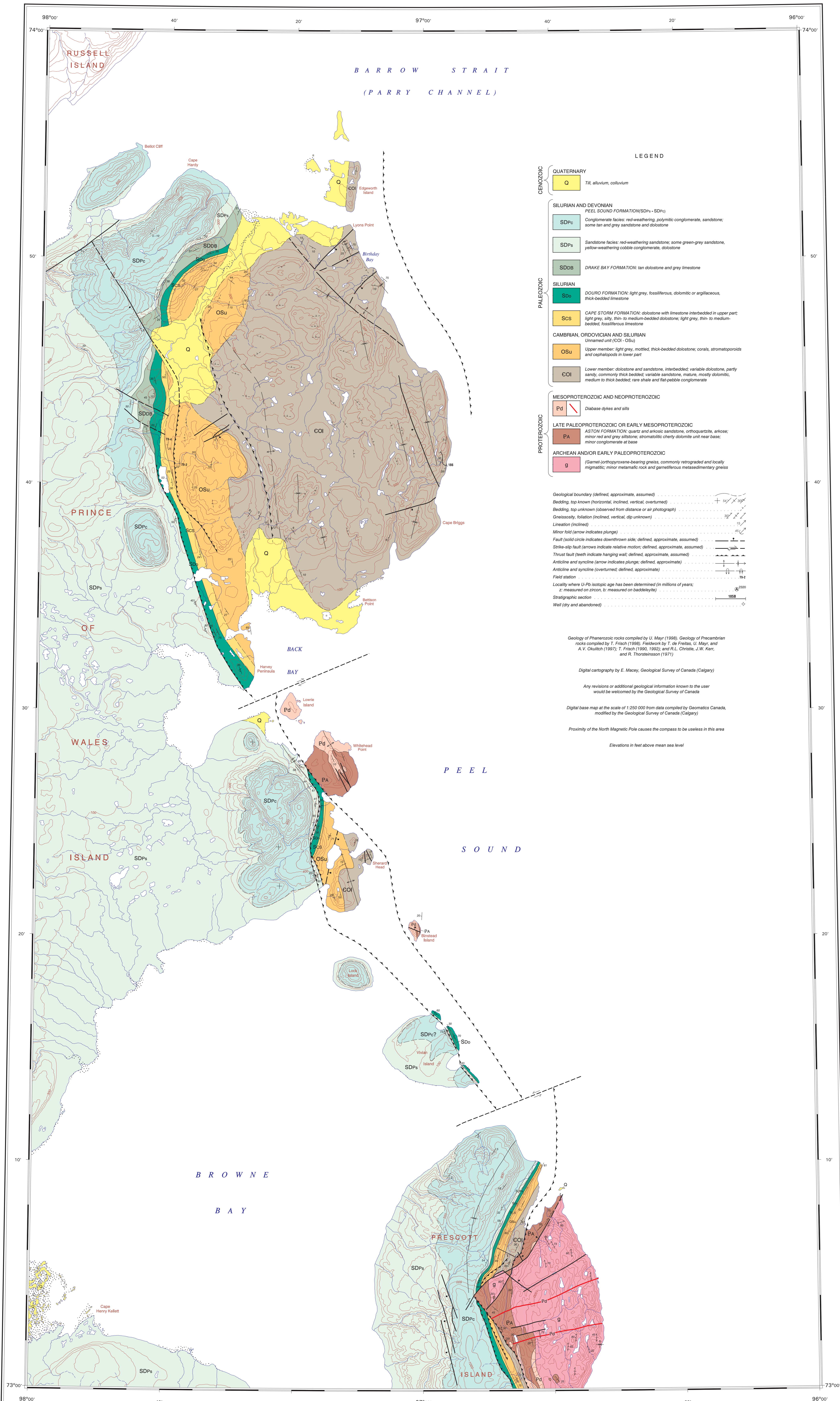
MAP 2016A GEOLOGY EASTERN PRINCE OF WALES ISLAND AND ADJACENT SMALLER ISLANDS NUNAVUT Scale 1:125 000/Echelle 1:125 000
