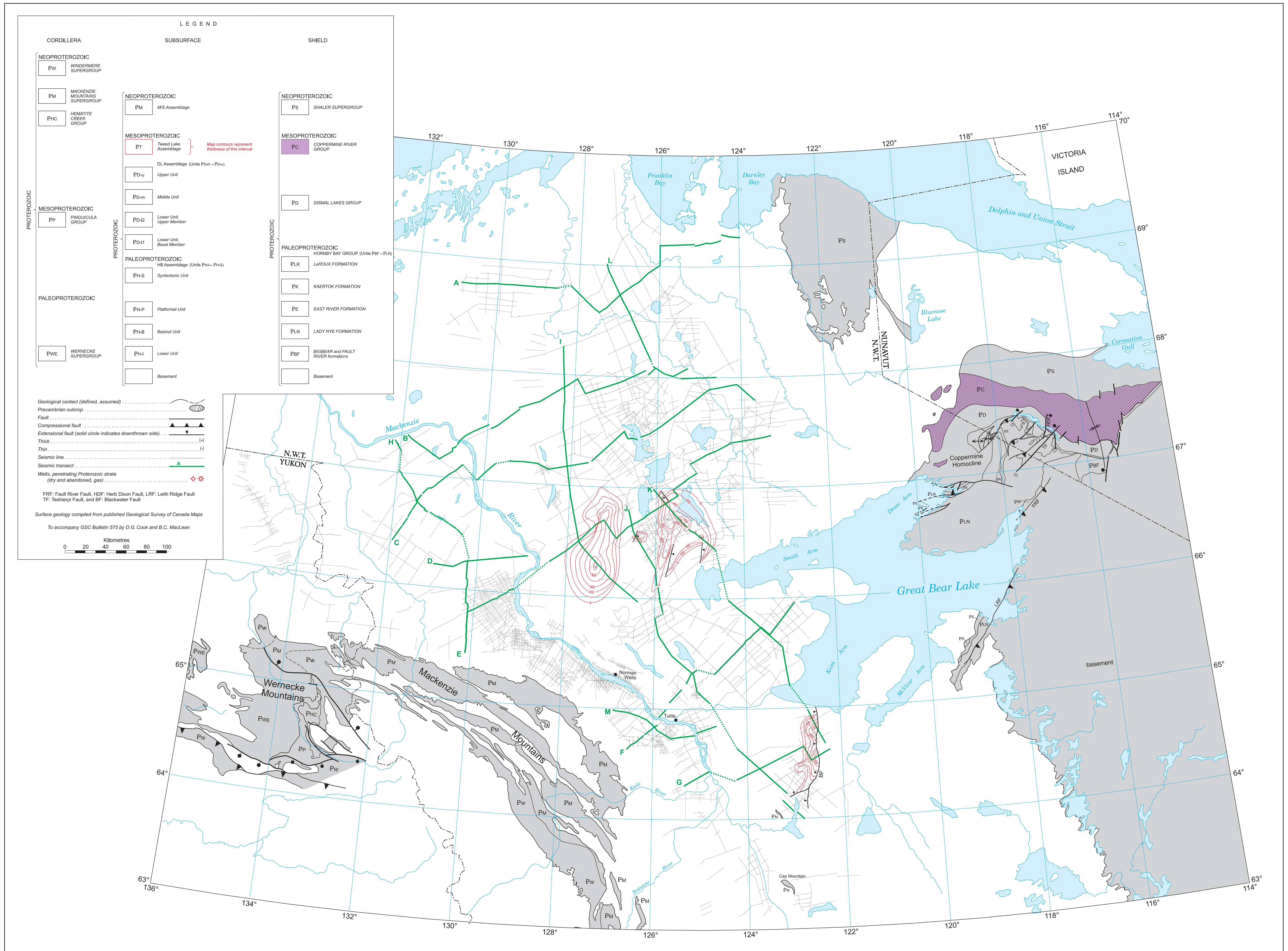
Figure 49. Seismic time-thickness map of the Tweed Lake Assemblage. Contour interval is 200 ms two-way time.
