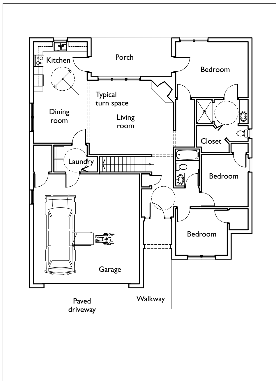
Figure 5 Example of an accessible house
