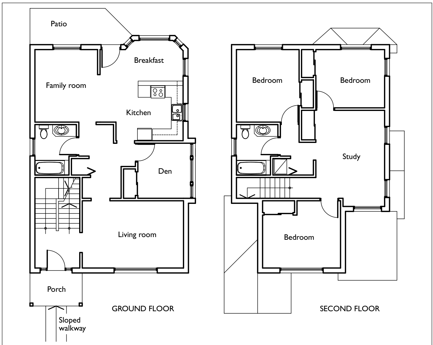
Figure 1 Example of a visitable house
