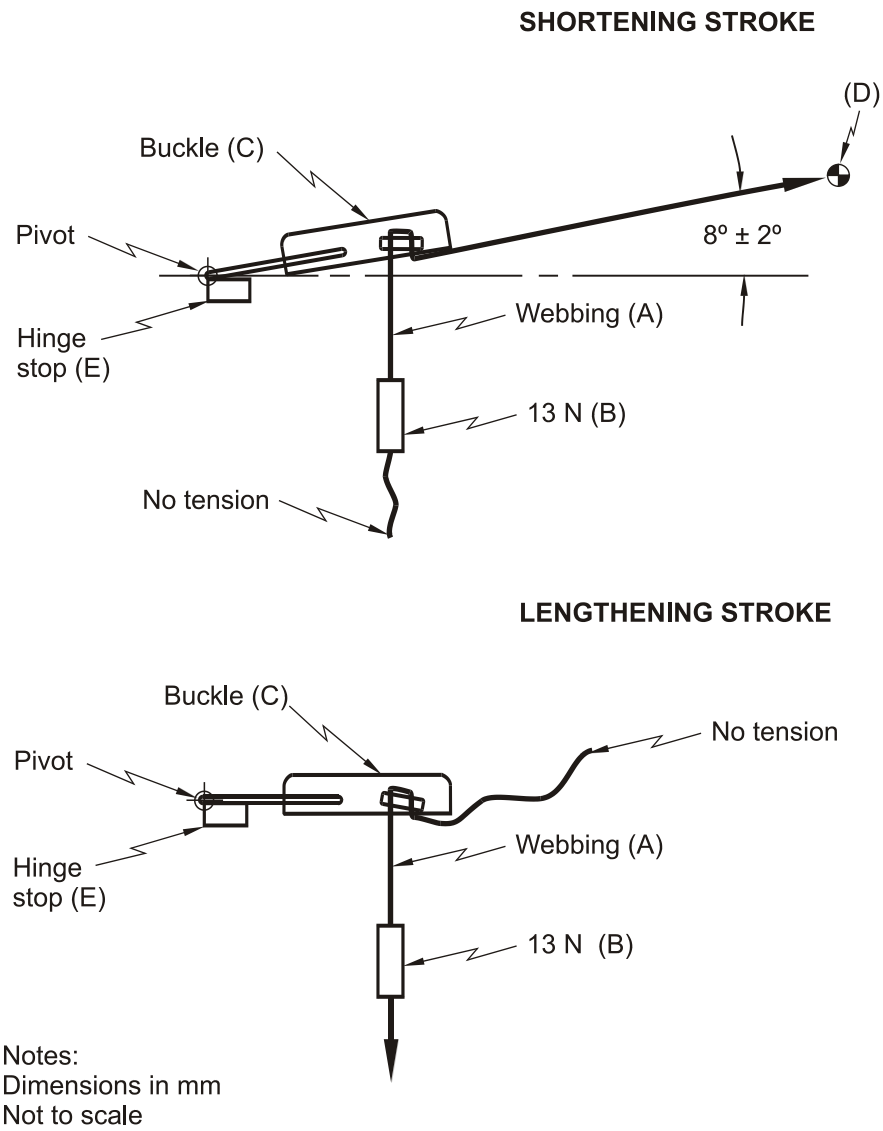
Figure 7 — Testing of Buckle Resistance to Abrasion
