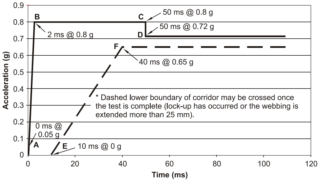
Figure 8 — Acceleration Corridors
