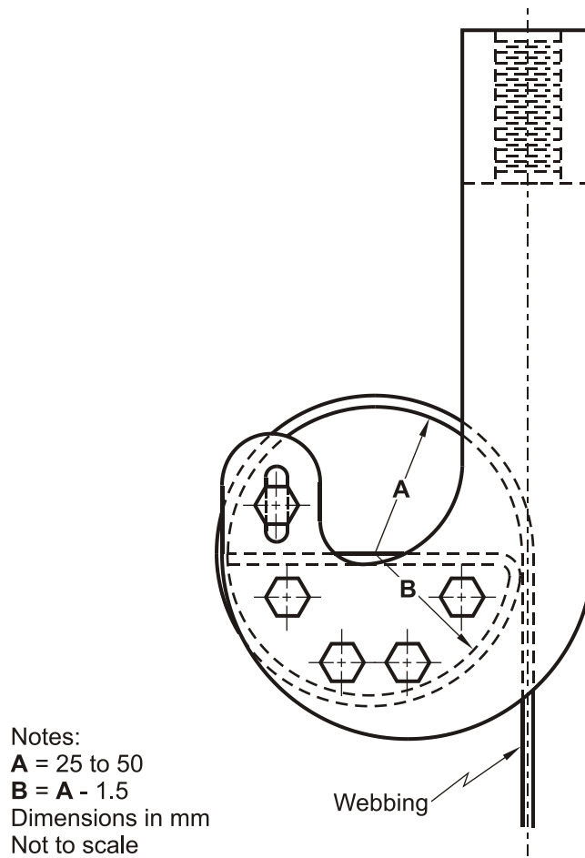
Figure 1 — Split Drum Grips to be Used for the Webbing Strength Tests
