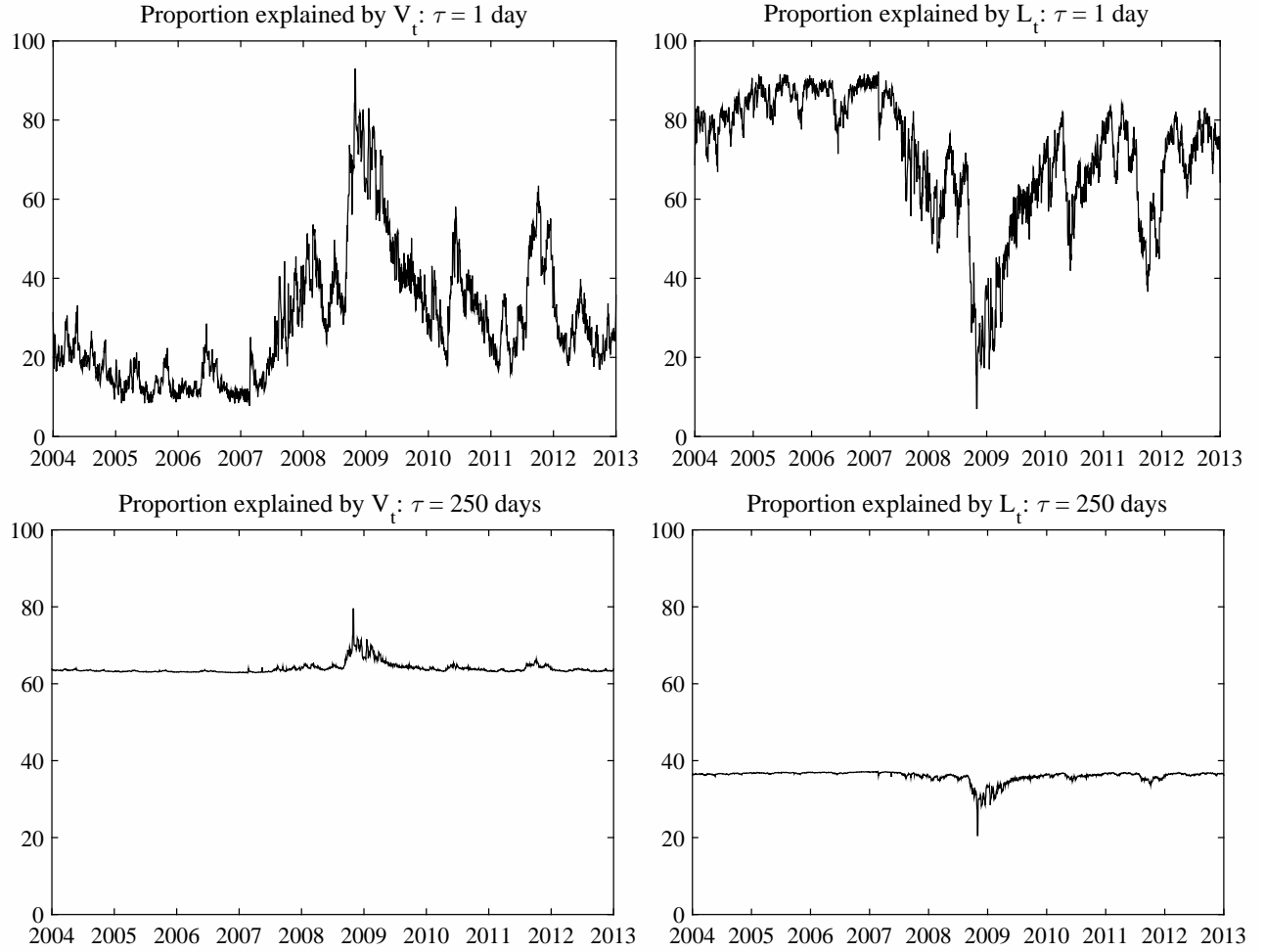
Figure 7: Proportion of Forecast Error Variance ( \hat{\epsilon}_{\lambda,t+\tau} ) Explained by V_t and L_t
