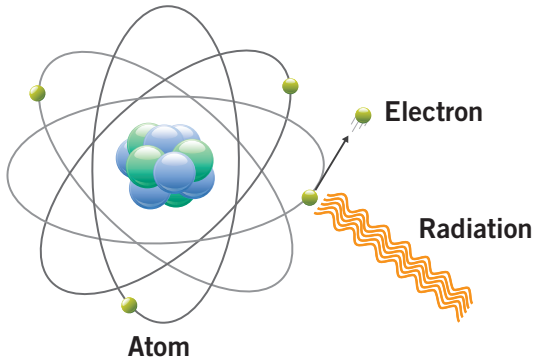
Figure 8: Ionisation.
