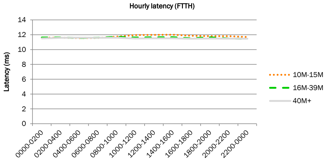
Figure 16: Hourly FTTH latency
