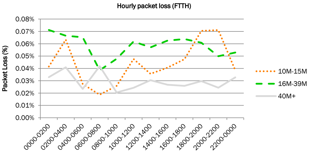
Figure 21: Hourly FTTH packet loss
