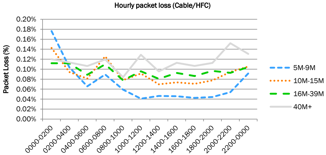
Figure 20: Hourly Cable/HFC packet loss
